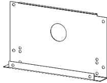
Right Cable Tray (1)
